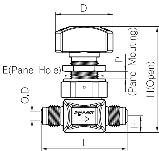
Male ZCR
