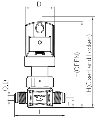
Male ZCR
