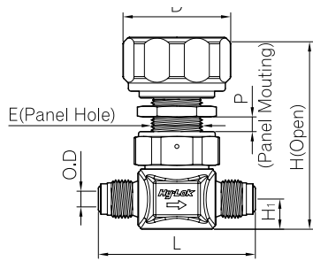
Male ZCR
